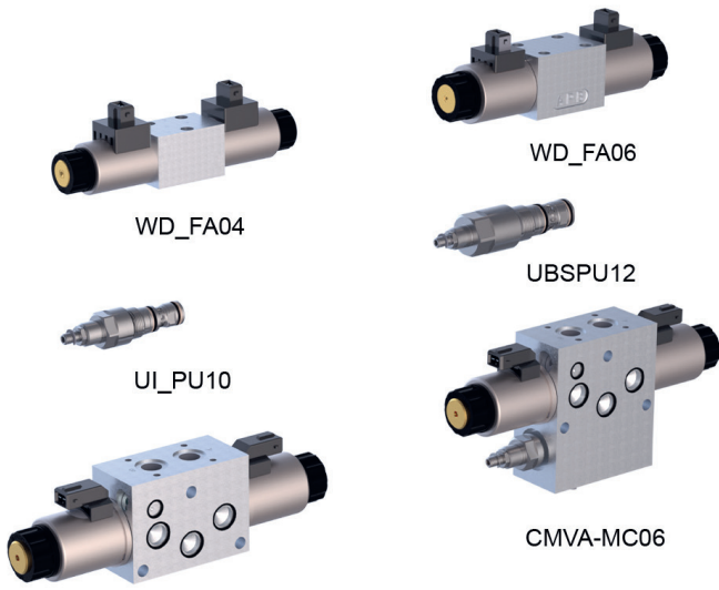
Examples of our components for tiltrotators
