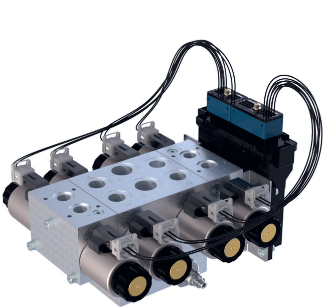
Tiltrotator solution consisting of the hydraulic control block with CAN bus capable electronics, based on a CMVA monoblock, complemented with two sectional CMVA-06 LS modules and our MD2 CAN controller.
