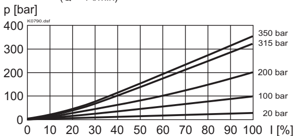
p = f(I) Pressure adjustment characteristics ( Q = 1 l/min)
