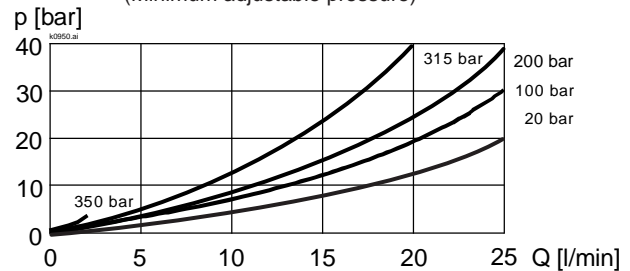
p = f(Q) Pressure volume flow characteristics (Minimum adjustable pressure)
